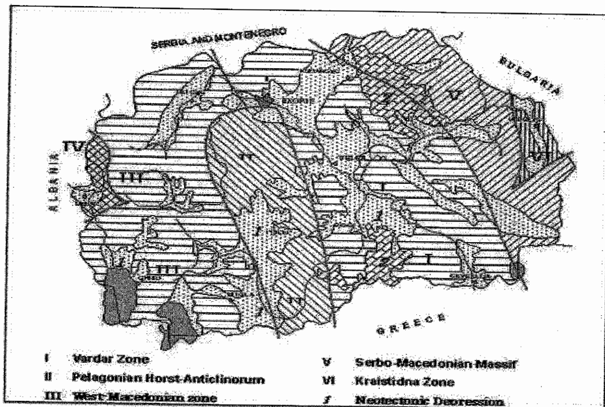
Fig. 1 Tectonic Zonation of Republic of Macedonia
